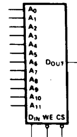
Figure 3. Logic Symbol
