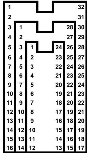
27xxx series EPROM Pinout Chart
